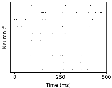
Spike trains
